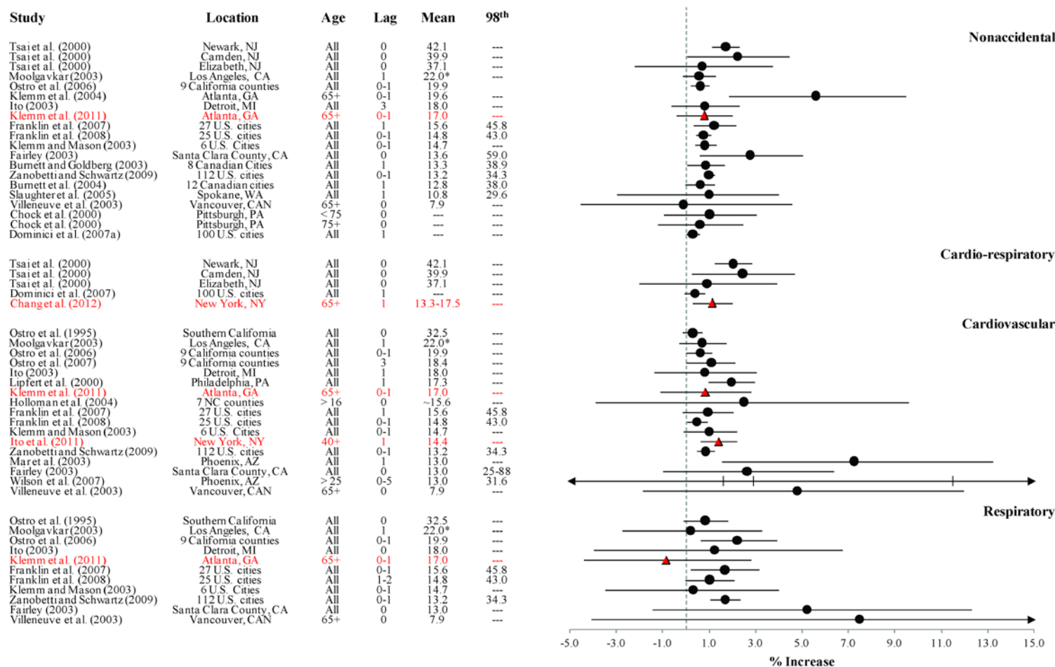
Figure 2.4 Percent increase in non-accidental and cause-specific mortality for a 10 µg/m 3 increase in 24-h average PM 2.5 concentrations in single-pollutant models from U.S. and Canadian studies. Red text and triangles represent recent studies published since the completion of the 2009 PM ISA.
