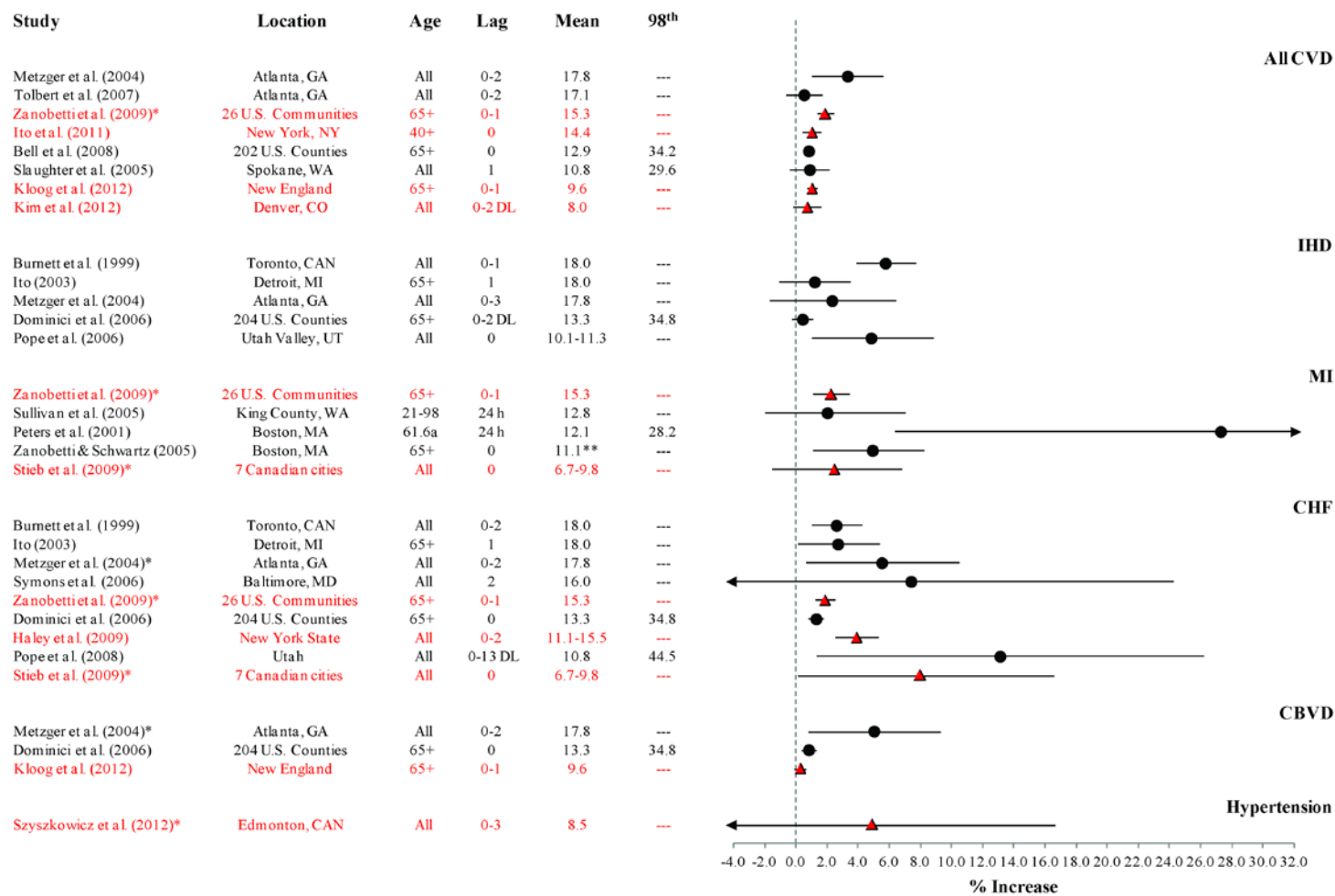
Figure 2.6 Percent increase in cardiovascular-related hospital admissions and ED visits for a 10 µg/m 3 increase in 24-h average PM 2.5 concentrations in single-pollutant models from U.S. and Canadian studies. Red text and triangles represent recent studies published since the completion of the 2009 PM ISA.
