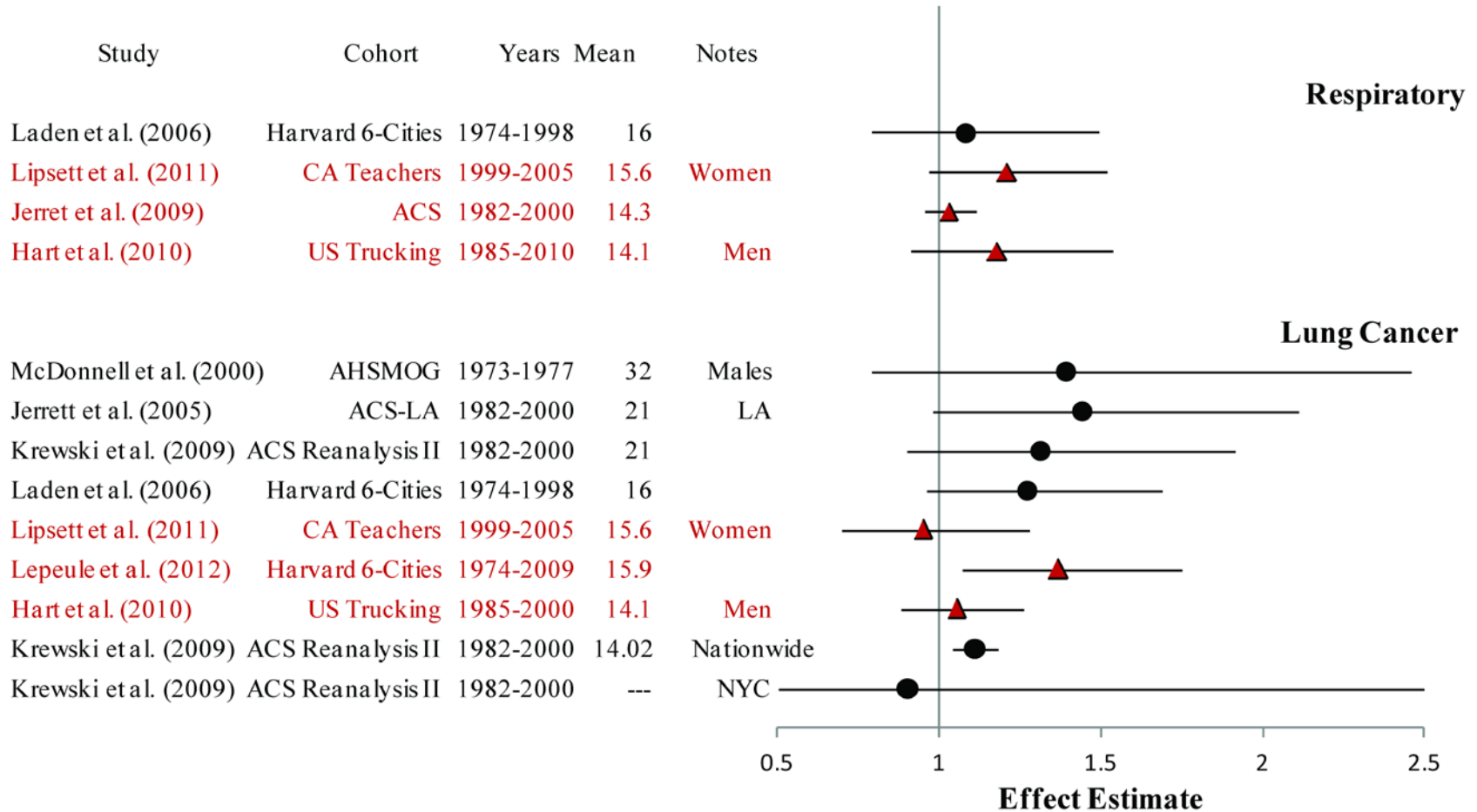
Figure 2.3 Respiratory mortality risk estimates, long-term exposure to PM_{2.5} in recent cohort studies. Red text and triangles represent new studies published since the completion of the 2009 PM ISA.
